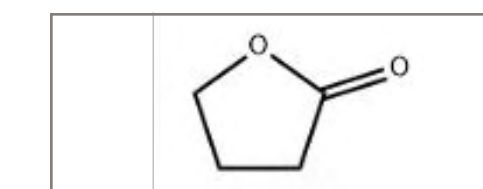
Gamma-Butyrolactone
