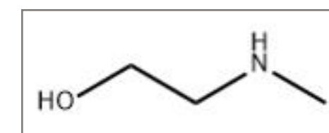
2-Methylaminoethanol
