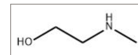
2-Methylaminoethanol
